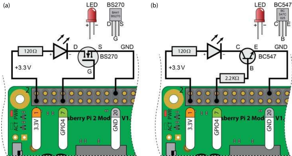
Figure 5-1: (a) Driving an LED with a GPIO using a FET, and (b) driving an LED with a GPIO using an NPN transistor
