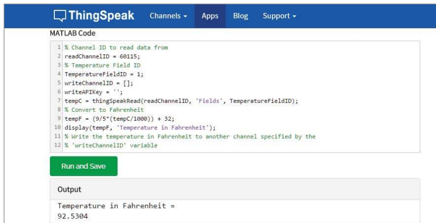
Figure 12-10: A ThingSpeak MATLAB example
