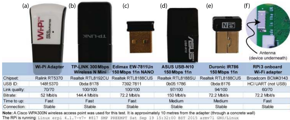
Figure 13-4: A selection of Wi-Fi adapters and test results when they are connected to the RPi
