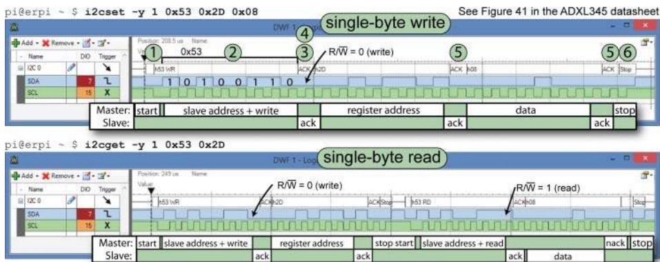
Figure 8-6: Capture and timings required for communication with the ADXL345 device
