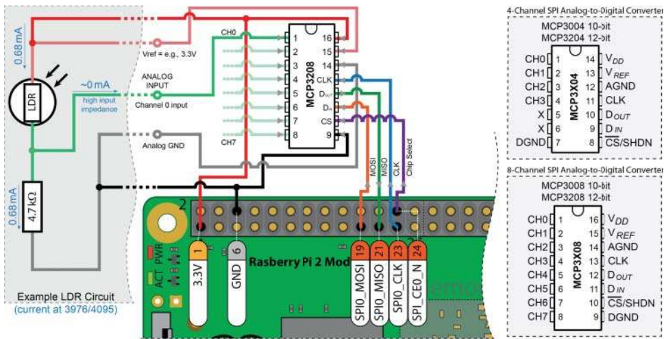
Figure 9-2: A general SPI ADC configuration for the RPi with an example LDR circuit attached to Channel 0 of the MCP3208 IC
