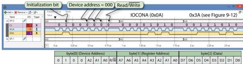
Figure 9-16: An SPI write request to the MCP23S17 at device address 000 to set the IOCONA register to 0x3A
