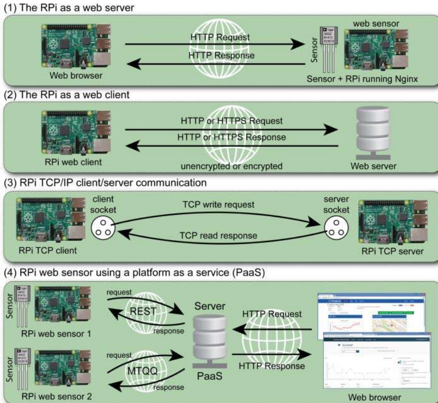
Figure 12-1: Different software communication architectures implemented in this chapter
