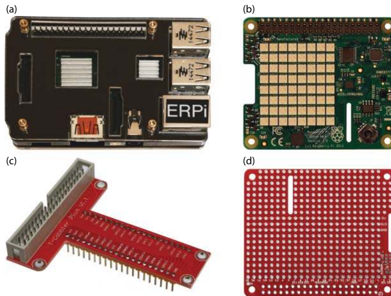
Figure 1-10: RPi Accessories: (a) An example case; (b) The Sense HAT; (c) The T-Cobbler board; and (d) A prototyping HAT
