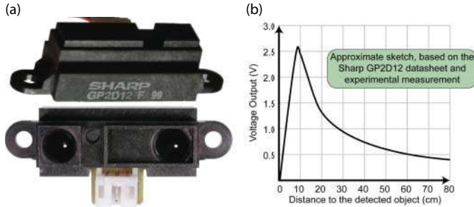
Figure 10-11: (a) Sharp infrared distance measurement sensor, and (b) its analog output response
