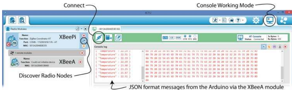
Figure 13-13: The XCTU Console working mode receiving JSON messages from the Arduino XBee device
