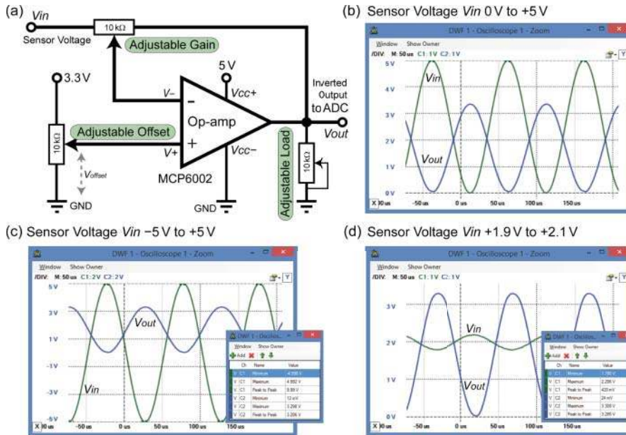
Figure 10-14: (a) A general op-amp signal conditioning circuit that inverts the input, (b) conditioned output when V_{in} is 0 V to 5 V, (c) conditioned output when V_{in} is -5\text{ V} to +5\text{ V} , and (d) conditioned and amplified output when the input signal is 1.9 V to 2.1 V
