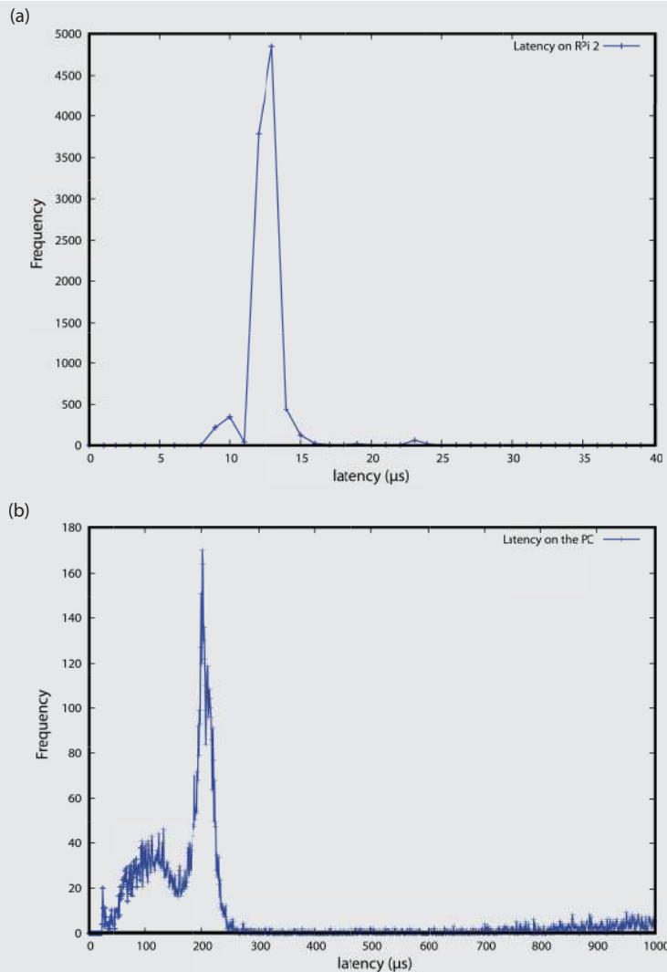
Figure 6-10: The cyclicttest results histogram for 10,000 samples (a) on the RPi 2, and (b) on a Linux desktop VM that is under load with no preemption support
